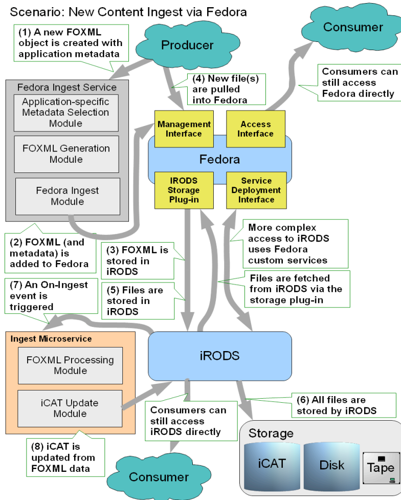
Figure 1: New Content Ingest via Fedora
