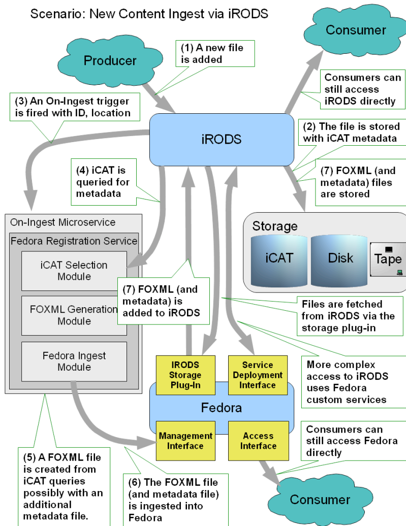
Figure 2: New Content Ingest via iRODS
